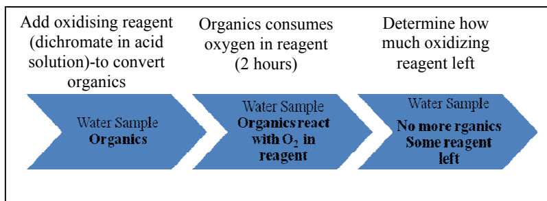
Fig. 4. Steps of the COD Test.
