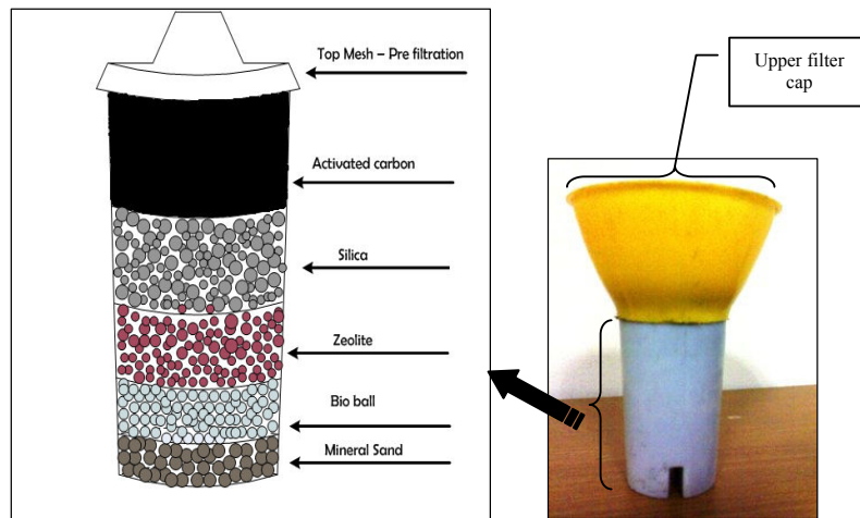
Fig. 2. Filter Cartridge and its Layers.
