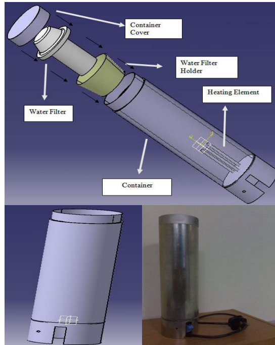
Fig. 3. Portable Water Filter Assembly.
